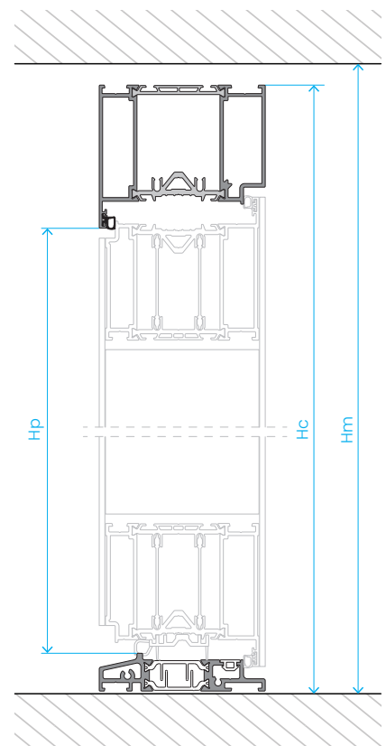
Vertical cross-section
