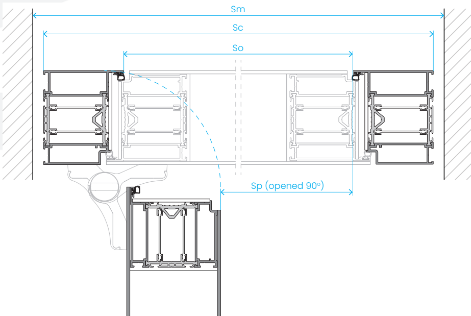
Horizontal cross-section
